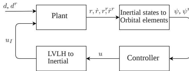
Figure 2. Block diagram of the closed-loop system (36)-(38), (40).
