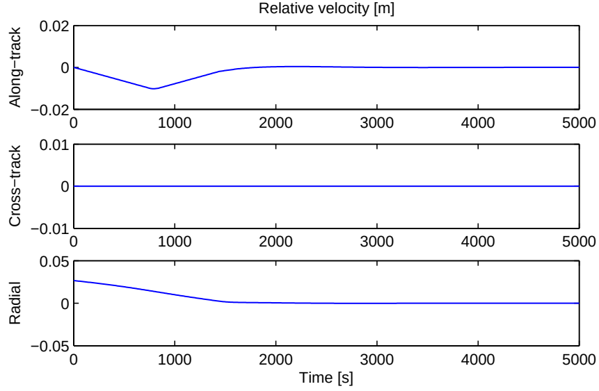
Figure 7. Relative velocity tracking error.
