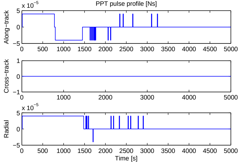
Figure 8. PPT impulse profile.
