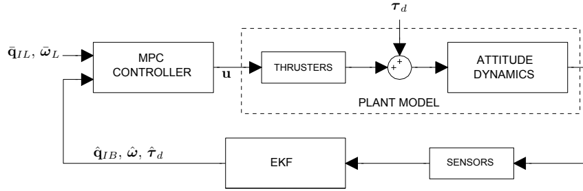
Figure 4. Closed-loop system
