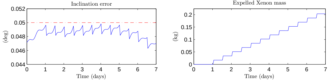
Figure 6. Weekly station-keeping cycle
