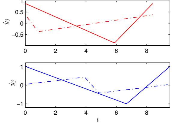
Fig. 5. Velocities \dot{y}_1(t) (solid) and \dot{y}_2(t) (dash-dotted) from the solution to (29) (top) and (33) (bottom).
