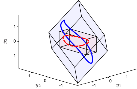
Fig. 8. Trajectories of the solution to (29) (dashed) and (33) (solid), together with constraints (17) (outer parallelotope) and |y_i| \leq a_i^* (inner box).
