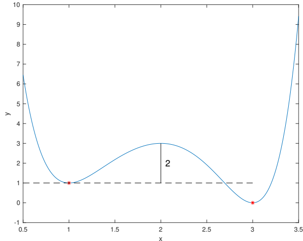
Figure 5: A function with two minima. The local minimum in x = 1 has prominence 2.
