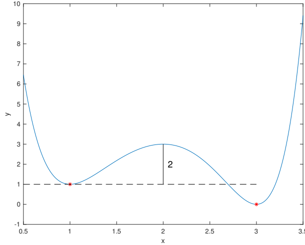
Figura 5: A function with two minima. The local minimum in x = 1 has prominence 2.
